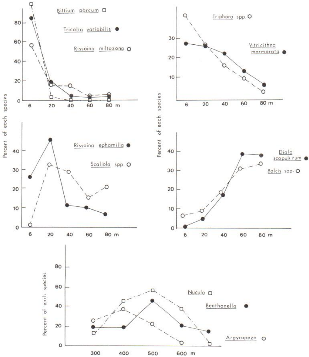
Figure 5.—Depth distribution of some commonly occurring micromollusks.
