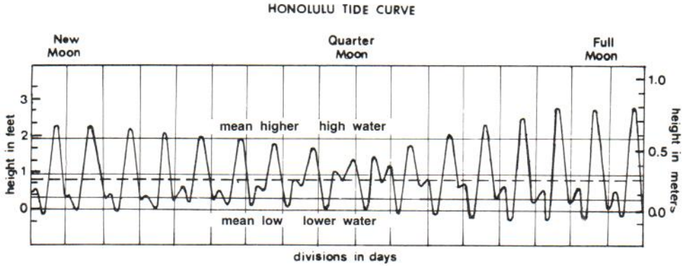
Figure 3.—Tide curves for Honolulu, Oahu. (From Atlas of Hawaii , p. 52, Department of Geography, Univ. Hawaii, 1973, by permission of University Press of Hawaii.)
