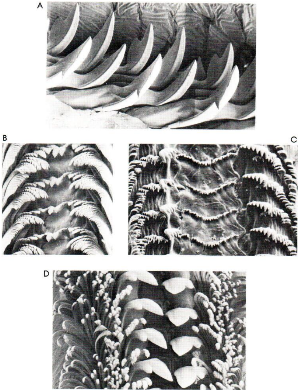
Figure 7.—Scanning electron microscope photographs of radulae. A. Docoglossate radula of Cellana exarata , 160X. Rhipidoglossate radulae of B. Tricolia variabilis , 380X. C. Sinezona insignis , 1500X. D. Diodora granifera , 160X.
