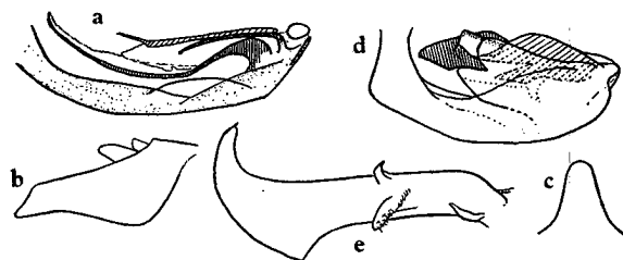
FIGURE 48.—a-c, Nesorhamma chalcas chalcas : a, aedeagus; b, anal segment of male; c, medioventral process of pygofer. d, e, Lamenia candida : d, aedeagus; e, genital style.
