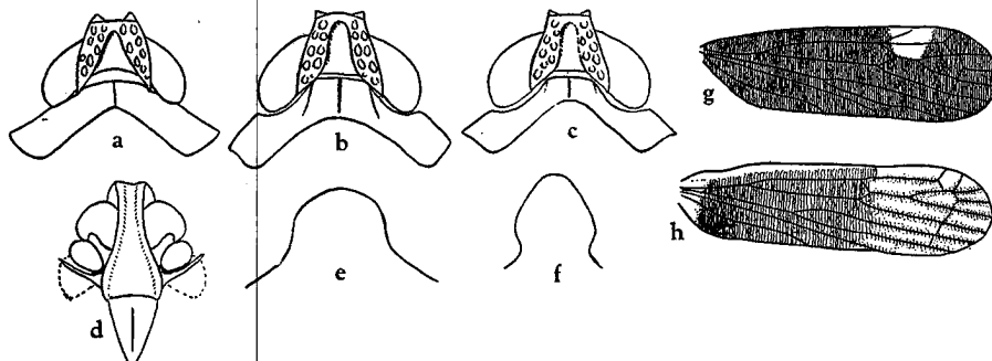
FIGURE 46.— a, f, g , Lamenia caliginea charon : a , vertex and pronotum; f , posterior margin of pregenital sternite of female; g , tegmen. b, e, h , L. numitor buto : b , vertex and pronotum; e , posterior margin of pregenital sternite of female; h , tegmen (Peleliu specimen); c, d , L. candida : c , vertex and pronotum; d , frons and clypeus.
