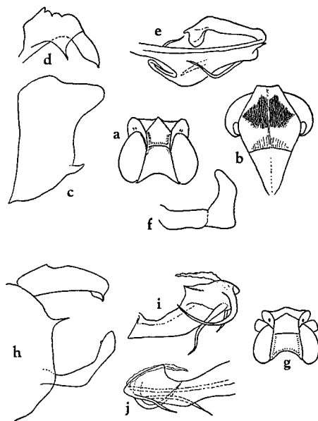
FIGURE 12.—a-f, Myndus ophiuchus : a, vertex; b, frons and clypeus; c, pygofer, left side; d, anal segment, left side; e, aedeagus, left side; f, left genital style. g-j, M. cressida : g, vertex; h, anal segment, pygofer, and genital style, left side; i, aedeagus, left side; j, aedeagus, right side.
