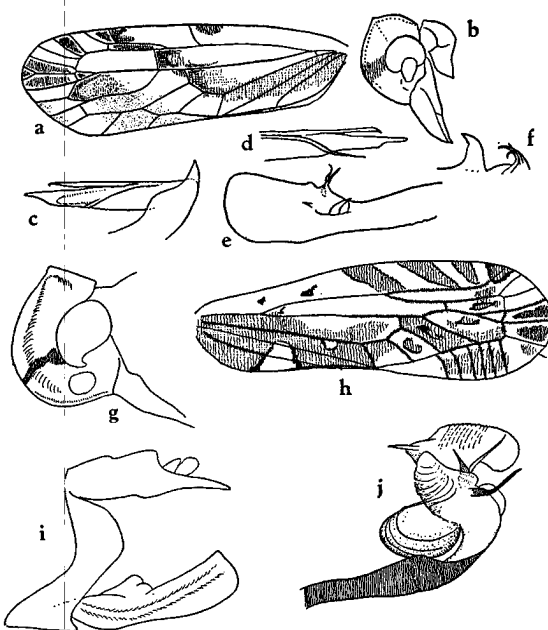
FIGURE 37.—a-f, Kamendaka (Eosaccharissa) lar : a, tegmen; b, head in profile; c, apical part of aedeagus, left side; d, apical part of aedeagus, right side; e, genital style; f, processes of genital style. g-j, K. (E.) polyphemus : g, head, side view; h, tegmen; i, anal segment, pygofer, and genital style, left side; j, aedeagus, left side.
