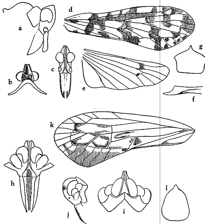
FIGURE 35.—a-g, Heronax achilles : a, head, pronotum, and dorsal profile of mesonotum, right side; b, head and pronotum, dorsal view; c, frons and clypeus; d, tegmen; e, wing; f, pregenital sternite, side view; g, pregenital sternite, ventral view. h-l, Paralyricen soranus : h, frons and clypeus; i, vertex and pronotum; j, head in profile; k, tegmen; l, pregenital sternite of female.
