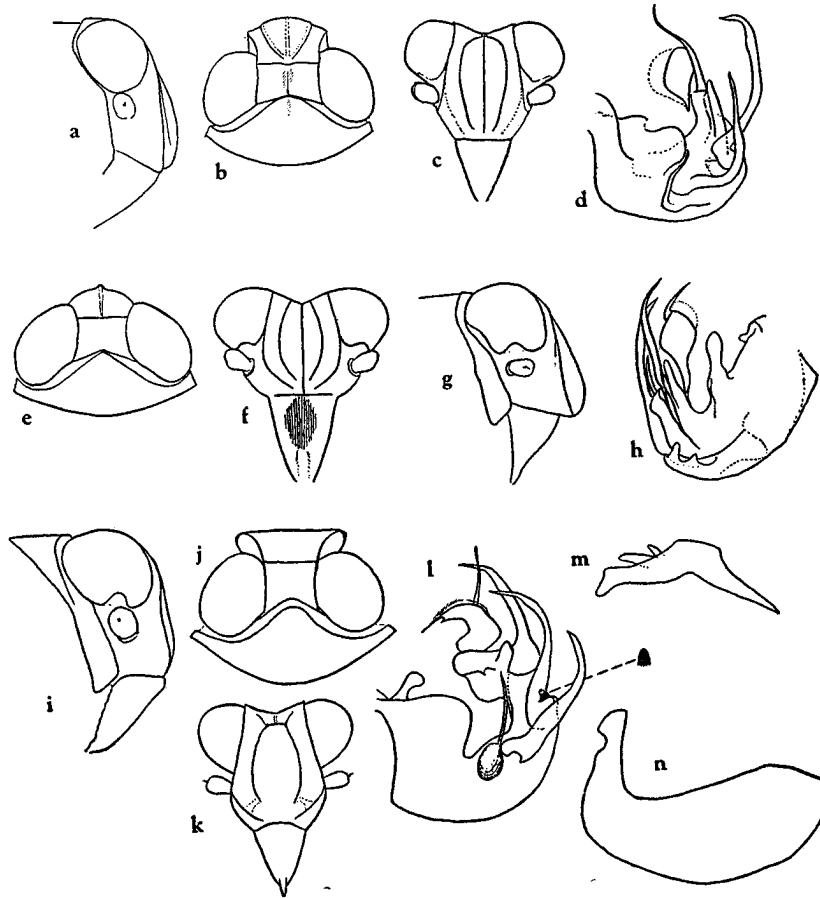
FIGURE 58.—a-d, Issarius carolinensis nassa : a, head in profile; b, vertex and pronotum; c, frons and clypeus; d, aedeagus. e-h, I. surenas : e, vertex and pronotum; f, frons and clypeus; g, head in profile; h, aedeagus. i-n, I. doricha : i, head in profile; j, vertex and pronotum; k, frons and clypeus; l, aedeagus; m, anal segment of male; n, genital style.
