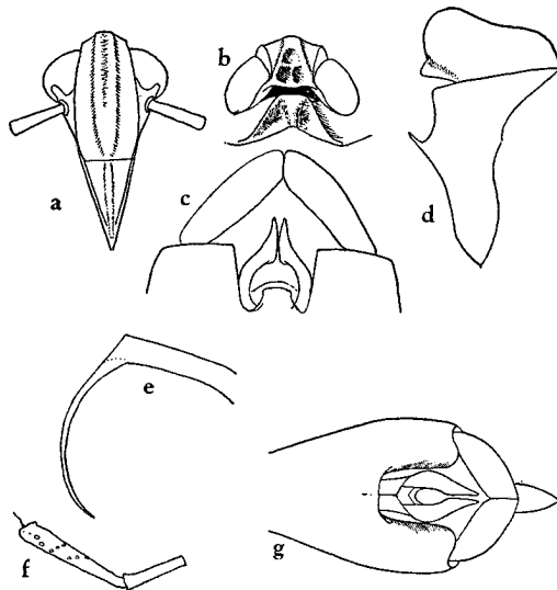
FIGURE 25.—a-f, Melanesia similior : a, frons and clypeus; b, head and pronotal disc; c, male genitalia, posteroventral view, aedeagus omitted; d, anal segment and pygofer, right side; e, aedeagus, ventral view; f, antenna. g, M. brevipennis : male genitalia, ventral view (drawn from specimen marked "type" in U. S. Nat. Mus.).
