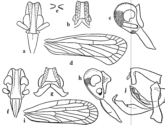
FIGURE 41.—a-e, Eusyphax bivittatus ianthe : a, frons and clypeus; b, vertex; c, head in profile; d, tegmen; e, processes adjoining apical margin of pregenital sternite. f-j, E. b. lineatus : f, frons and clypeus; g, vertex and pronotum; h, head and pronotum in profile; i, tegmen; j, male genitalia.
