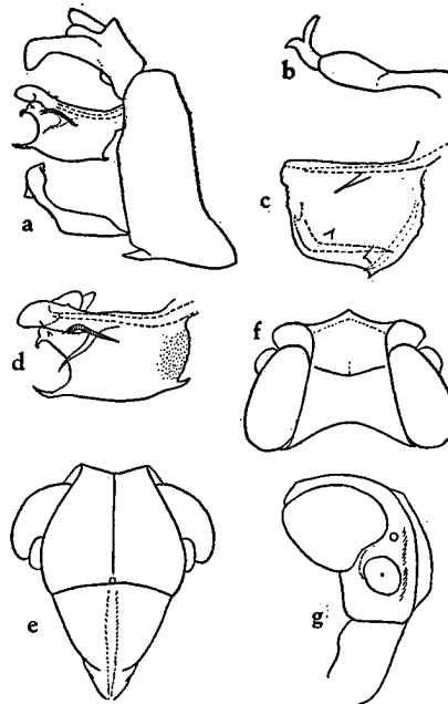
FIGURE 3.—a, d, Myndus polycator : a, male genitalia; d, aedeagus. b, c, M. bifurcatus : b, genital style; c, aedeagus. e-g, M. dibaphus : e, frons and clypeus; f, vertex; g, head in profile.
