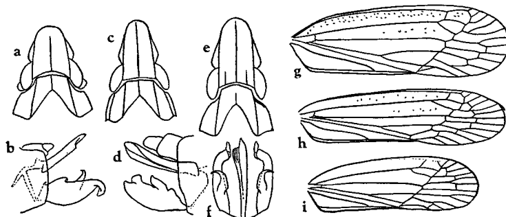
FIGURE 54.—a, d, g, Tambinia guamensis : a, vertex and pronotum; d, male genitalia, right side; g, tegmen. b, c, h, T. baucis : b, aedeagus; c, vertex and pronotum; h, tegmen. e, f, i, T. sisypus : e, vertex and pronotum; f, aedeagus and genital style, ventral view; i, tegmen.
