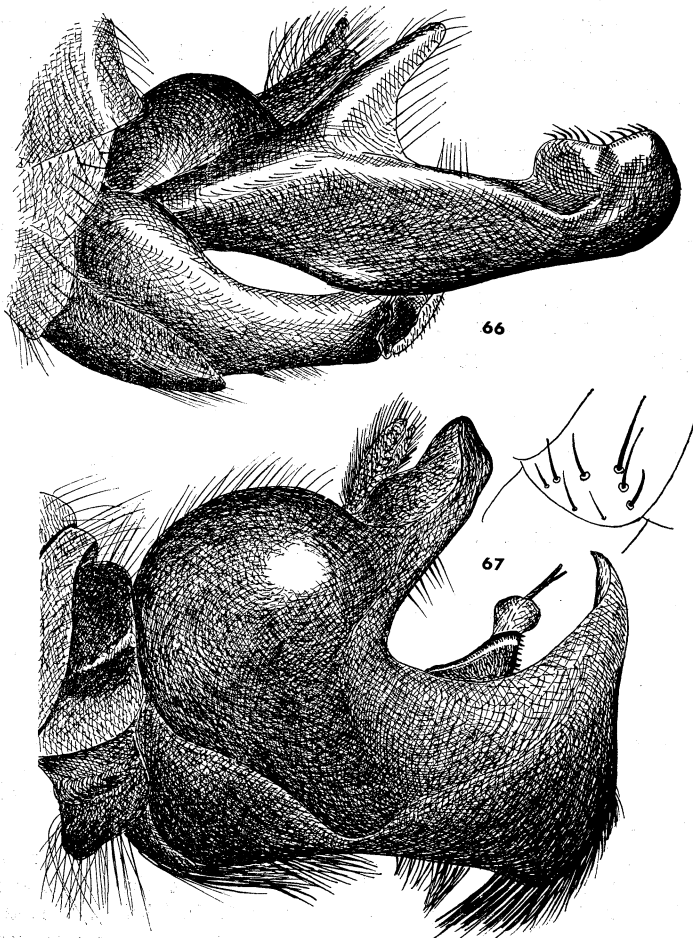
Fig. 66, 67. Heligmoneura , ♂ genitalia. 66, spreti (Wulp); 67, sula n. sp., inset, upturned bristles on sixth tergite.
