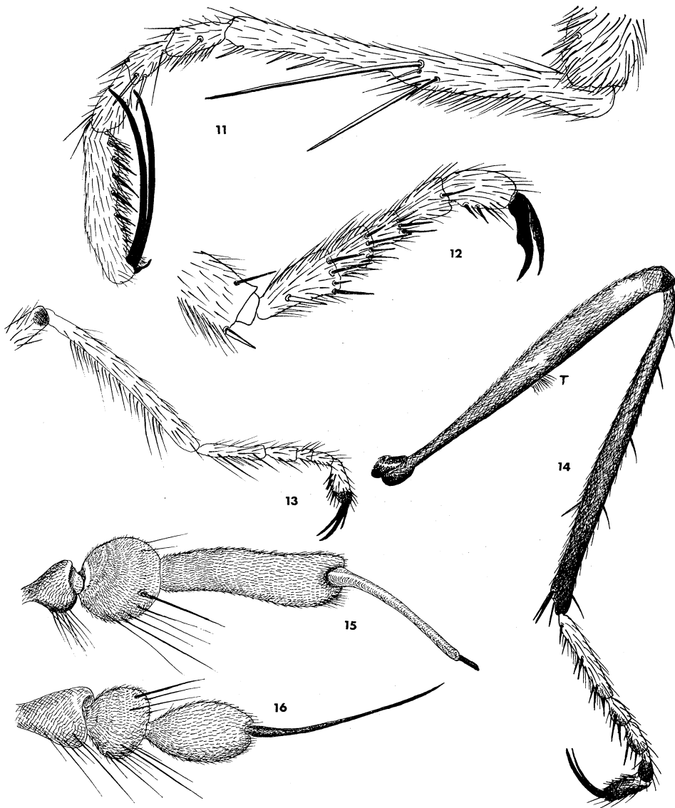
Fig. 11-16. 11-14, details of leg-structure: 11, Euscelidia piliensis n. sp., fore tarsus (cf. with setifer (Frey)); 12, Leptogaster crassicarsis Frey, hind tarsus; 13, Leptogaster cilipes Frey, fore leg; 14, Ammophilomima boettcheri Frey, hind leg; note ventral tuft, T. 15, 16, antennae: 15, Euscelidia setifer (Frey); 16, Euscelidia piliensis n. sp.
