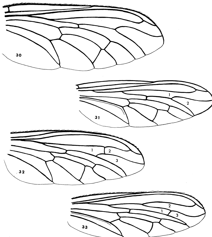
Fig. 30-33. Wings: 30, Orthogonis scapularis (Wiedemann), wing color omitted; 31, Andrenosoma irigensis n. sp.; 32, Pogonosoma cyanogaster Bezzi; 33, Pogonosoma basifera (Walker). Numbers 1-3=submarginal cells.
