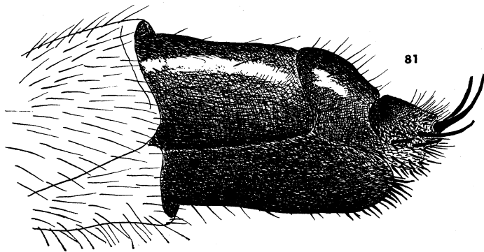
Fig. 80, 81. Philonicus nigrosetosus Wulp : 80, ♂ genitalia in dorsal view ; 81, ovipositor in lateral view.
