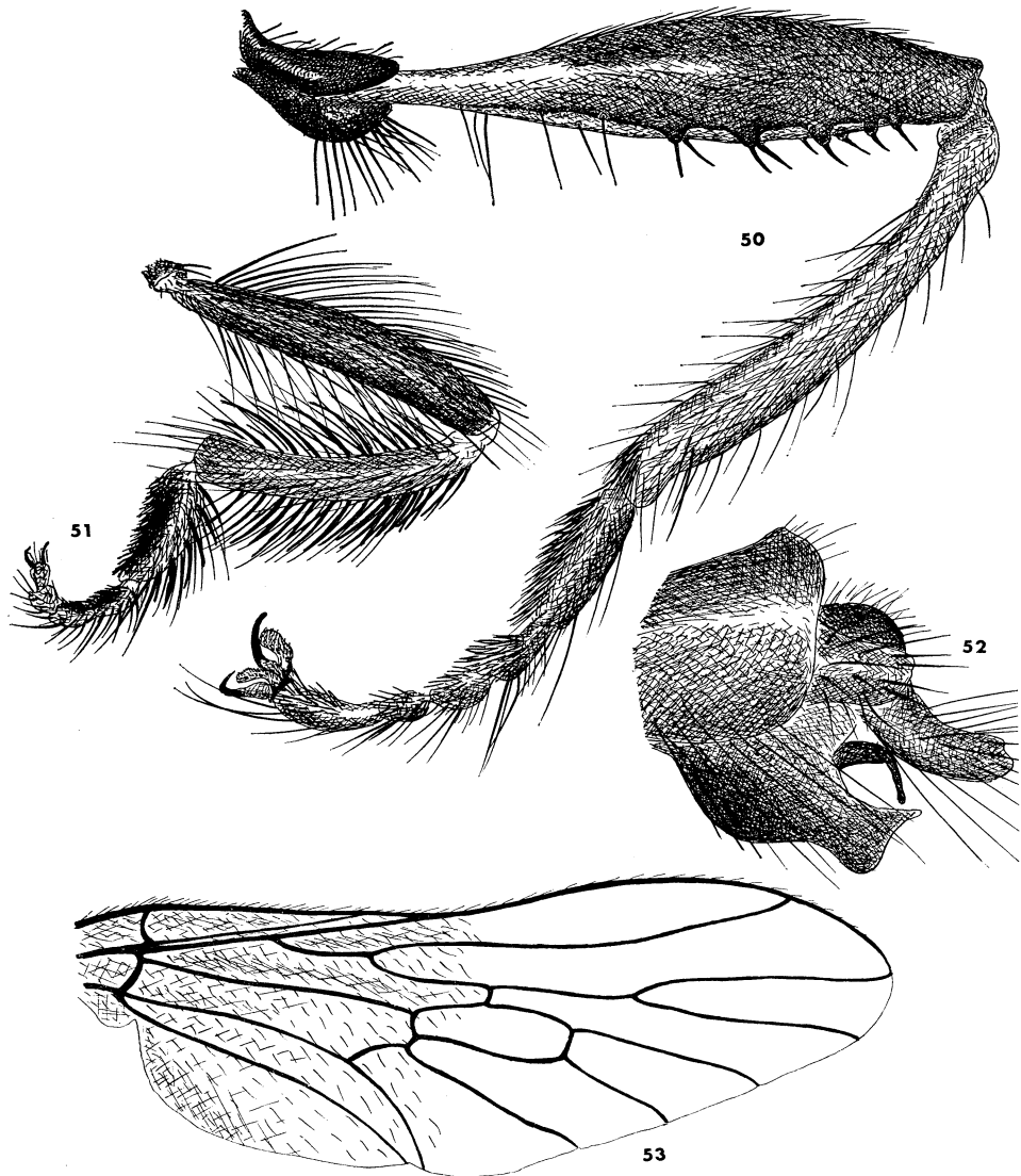
Fig. 50-53. Xenomyzini. 50, Xenomyza vitripennis (Osten Sacken), left hind leg of ♂; 51, Trigonomima cyanella (Osten Sacken), hind leg of ♂; 52, Damalina semperi Osten Sacken, ♂ genitalia; 53, Trigonomima cyanella (Osten Sacken).
