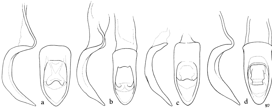
Fig. 10. Pantorhytes aedeagi, as in figure 1: a, verrucatus (Bates), New Britain; b, brandti n. sp.; c, torricellianus Hllr, Torricelli Mts; d, sexpustulatus Hllr, Finisterre Mts.
