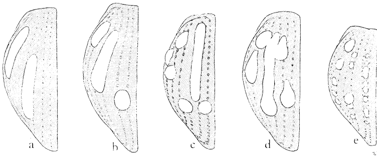
Fig. 17. Pantorhytes elytral diagrams: a, obliquus n. sp.; b, vibicifer Hllr, Goilala; c, ?papuanus Gestro, Karimui, NE NG; d, rubroverrucatus (Tryon), Inauwauni; e, polynodus n. sp.
