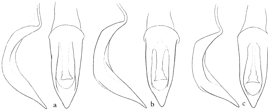
Fig. 6. Pantorhytes aedeagi, as in figure 2: a, b, batesi Faust, Markham Valley; b, proximus Faust Papua; c, plutus (Ober.). New Britain.
