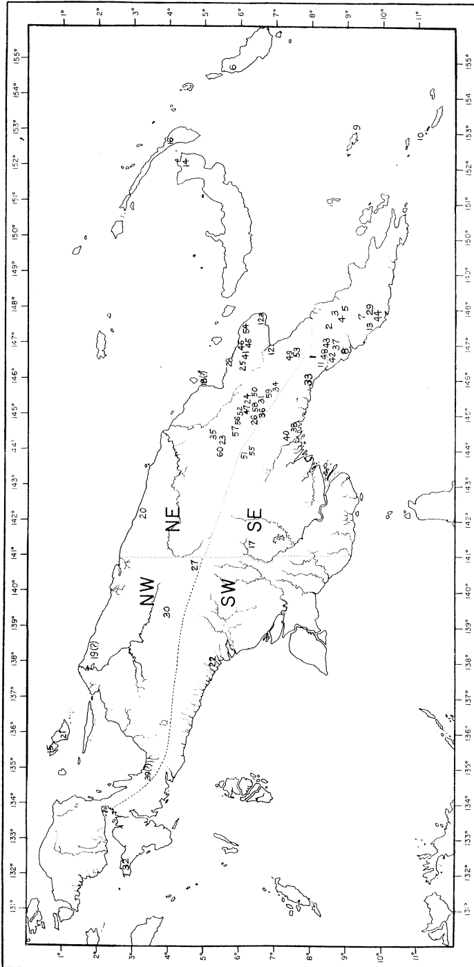
Fig. 1. Map of New Guinea showing locations of type localities of Pantorhytes .
