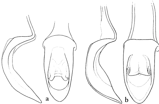
Fig. 16. Pantorhytes aedeagi, as in figure 2: a, vibicifer Hllr, Goilala; b, polynodus n. sp.
