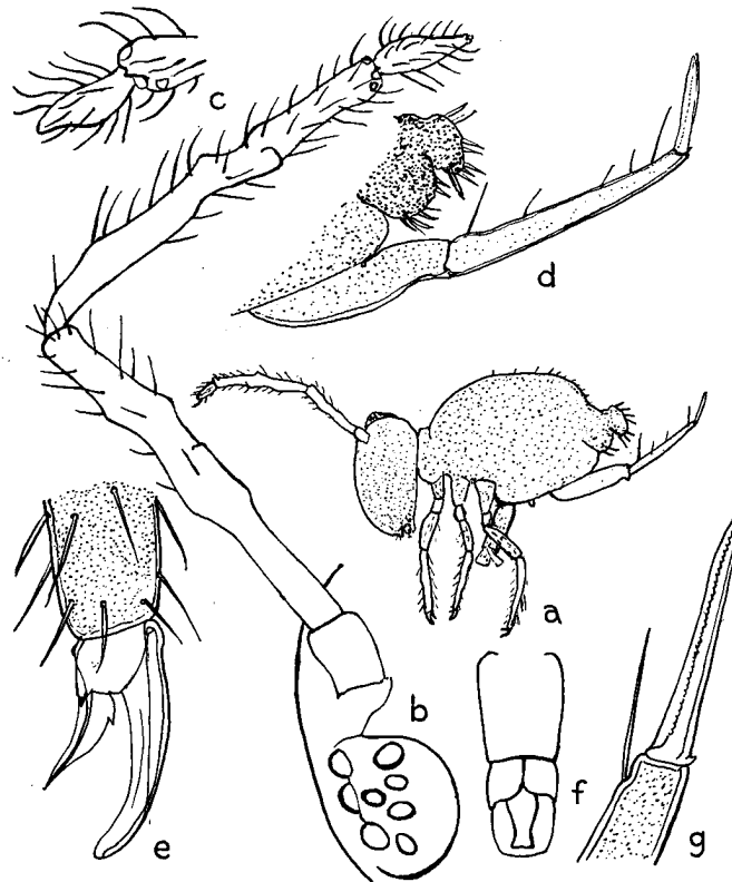
FIGURE 7. Dicyrtoma insularis , new species: a, side view, \times 43 ; b, left feeler and ocular area, \times 160 ; c, tip of right feeler, \times 200 ; d, hind region of abdomen and spring, side view, \times 133 ; e, hind foot, \times 453 ; f, ventral tube, front view, \times 133 ; g, terminal part of dens, and mucro, \times 266 .
