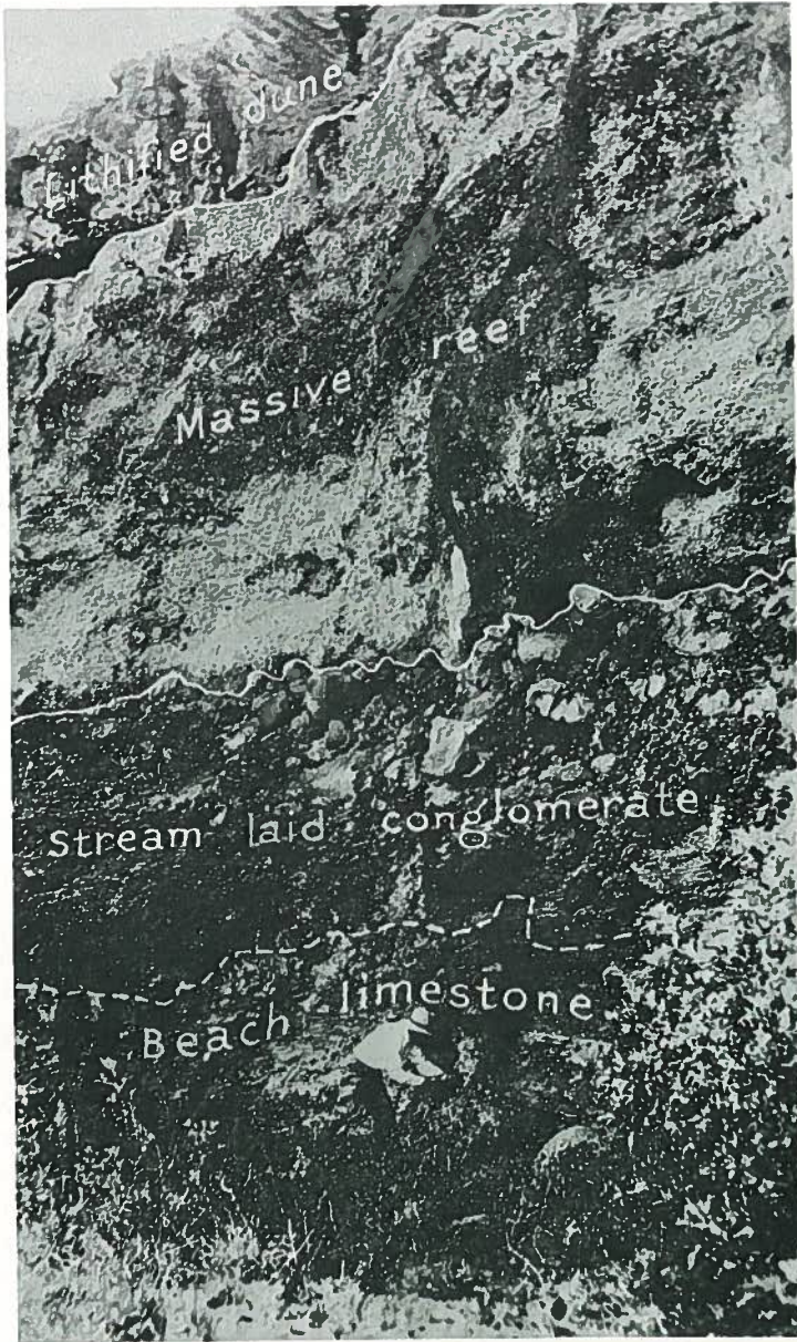
FIGURE 6. —Cliff near Kahuku, Oahu, showing the beach limestone of the Kahuku Point 55-foot shoreline separated by an erosional unconformity from the stream-laid conglomerate of Kahipa age. Another unconformity separates the conglomerate from the massive reef of Kaena age and it is, in turn, separated by soil and a solution unconformity from lithified dunes laid down during the Waipio low stand. Photo by H. T. Stearns.
