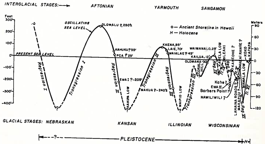
FIGURE 1.—Graph showing glacioeustatic fluctuations of sea level and Hawaiian Pleistocene shorelines.
