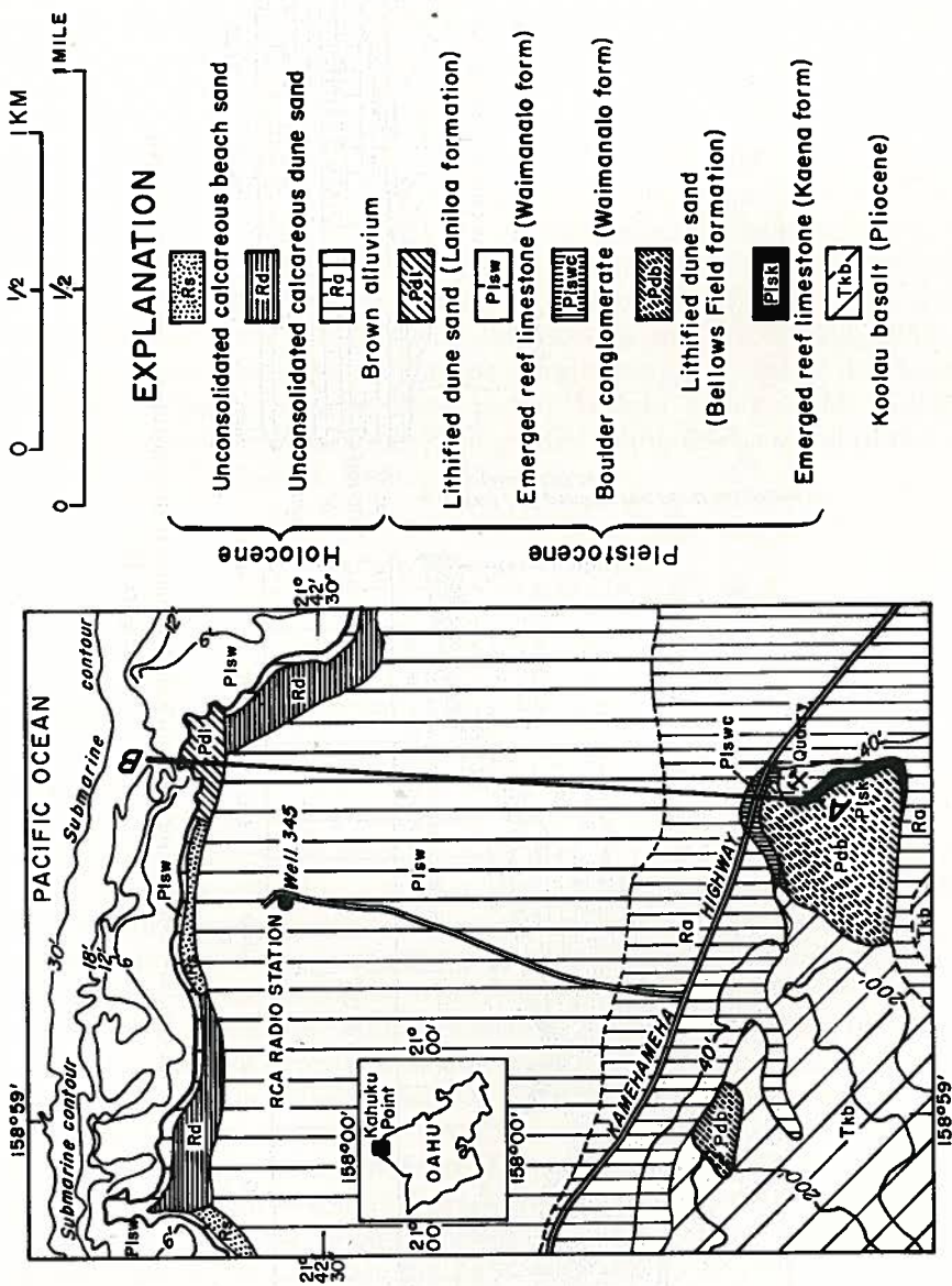
FIGURE 10.—Geologic map of Kahuku Point, Oahu.
