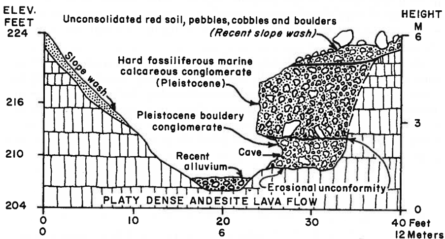
FIGURE 4.—Geologic section of marine conglomerate on Molokai island.
