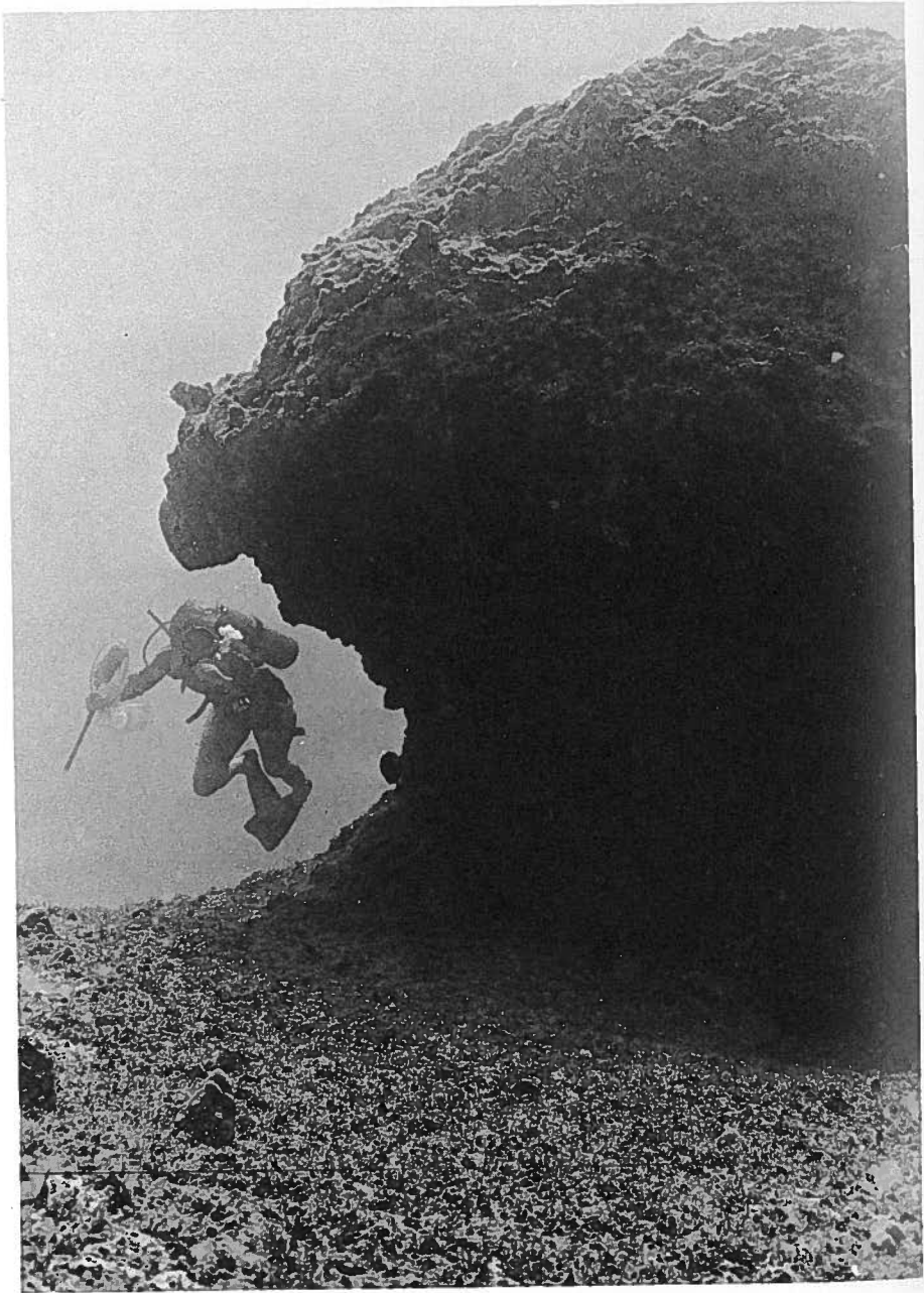
FIGURE 20.—View of notch of the -80-foot shoreline with overhanging visor in dead coral reef in Kaneohe Bay, Oahu. Photo by Robert Dill. Published by permission of the U.S. Navy.
