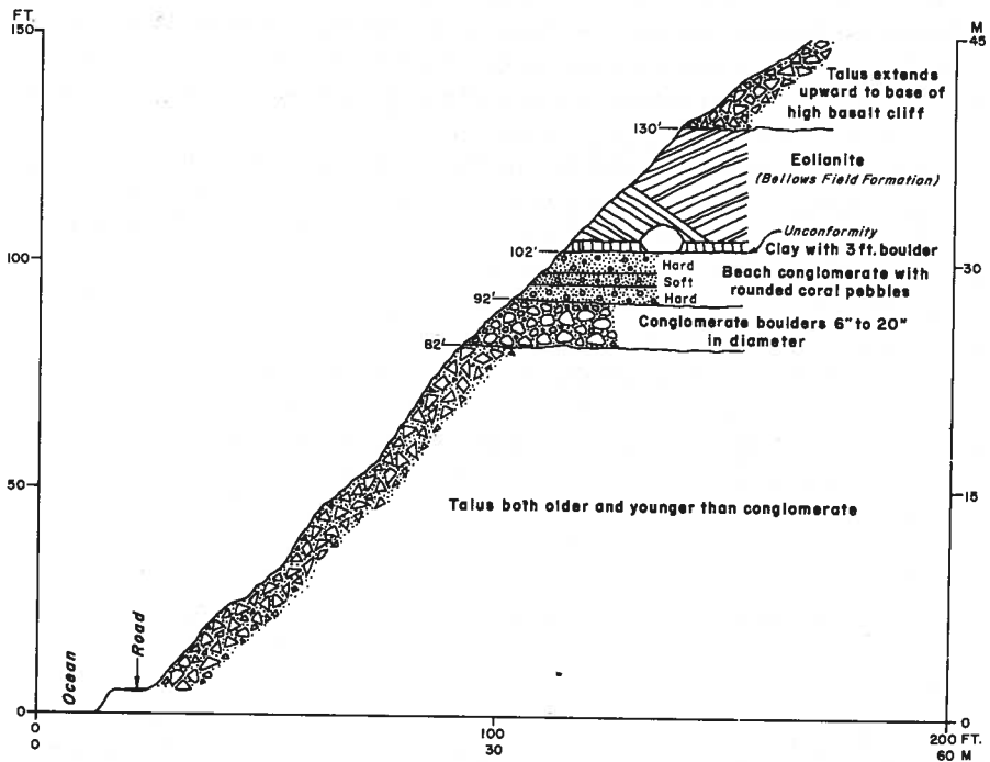
FIGURE 8.—Geologic section of Kaena beach deposits 1\frac{1}{4} miles southeast of Kaena Point, Oahu.
